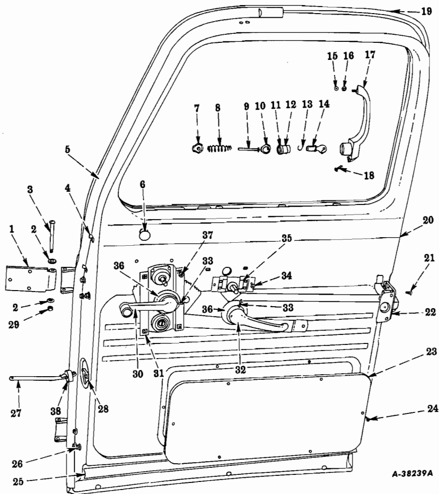
FIG. 16-24 – CAB DOOR ASSEMBLY (For Codes 1606, 1617, 1618, 1619) (R-100-19474, R-110-53455, R-120-11688, R-130-10102, R-140-4x4-1053, R-150-3844, R-160-32760, R-160-4x4-974, RC-160-2997 And Up)
