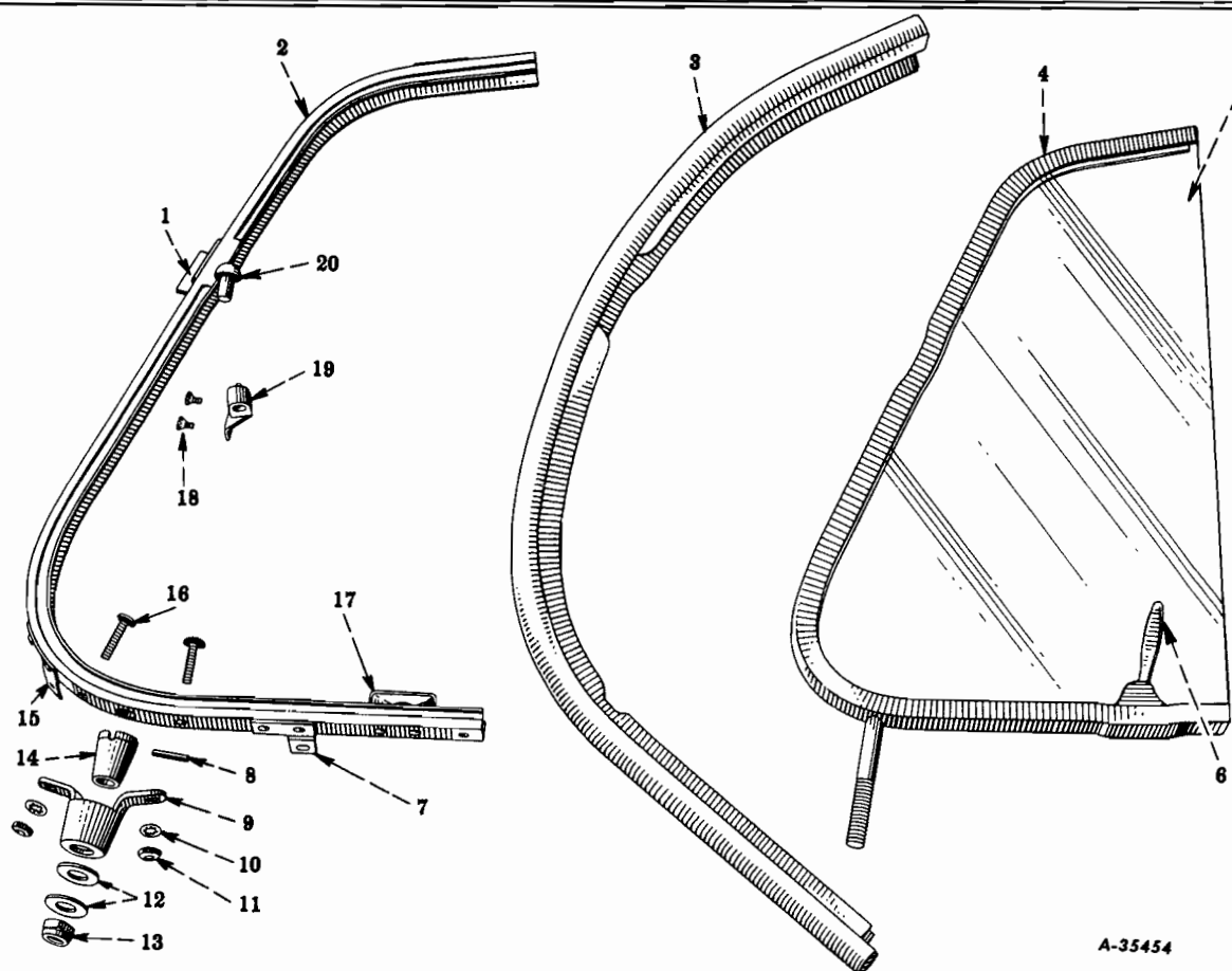
FIG. 16-28 — DOOR VENT WINDOW (Troy Sunshade) (For Codes 1603, 1610, 1613, 1616, 1617) (Below R-100-19474, R-110-53455, R-120-11688, R-130-10102, R-140-4x4-1053, R-150-3844, R-160-32760, R-160-4x4-947, RC-160-2997) (Optional With Fig. 16-27)
