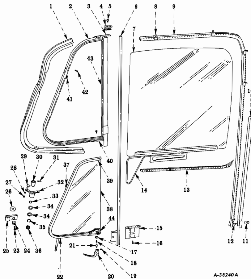
FIG. 16-26 – CAB DOOR WINDOW AND VENT WINDOW (For Codes 1606, 1617, 1618, 1619) (R-100-19474, R-110-53455, R-120-11688, R-130-10102, R-140-4x4-1053, R-150-3844, R-160-32760, R-160-4x4-974, RC-160-2997 And Up)
