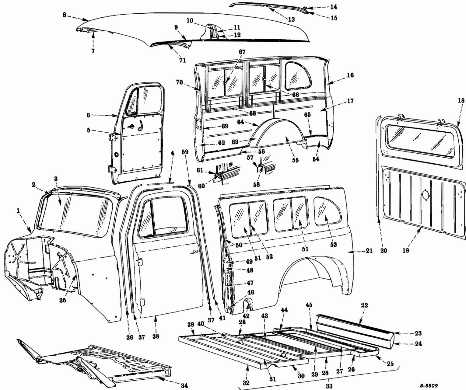
FIG. 16-43 — TRAVELALL BODY ASSEMBLY (For Travelall Body With Standard Liftgate and Tailgate Code 1616, 1619) (For Travelall Body With Double Rear Doors Code 1617)
