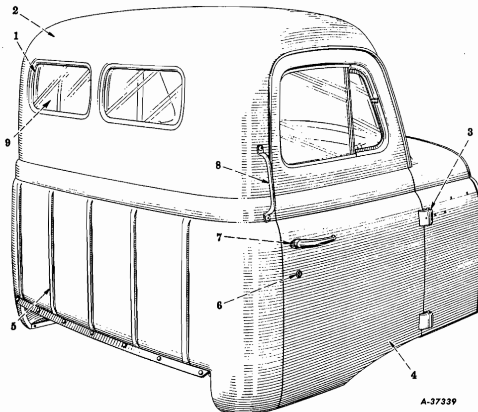
FIG. 16-13 - CAB ASSEMBLY (Codes 1606, 1613) (Right Rear View) (RC-160)
