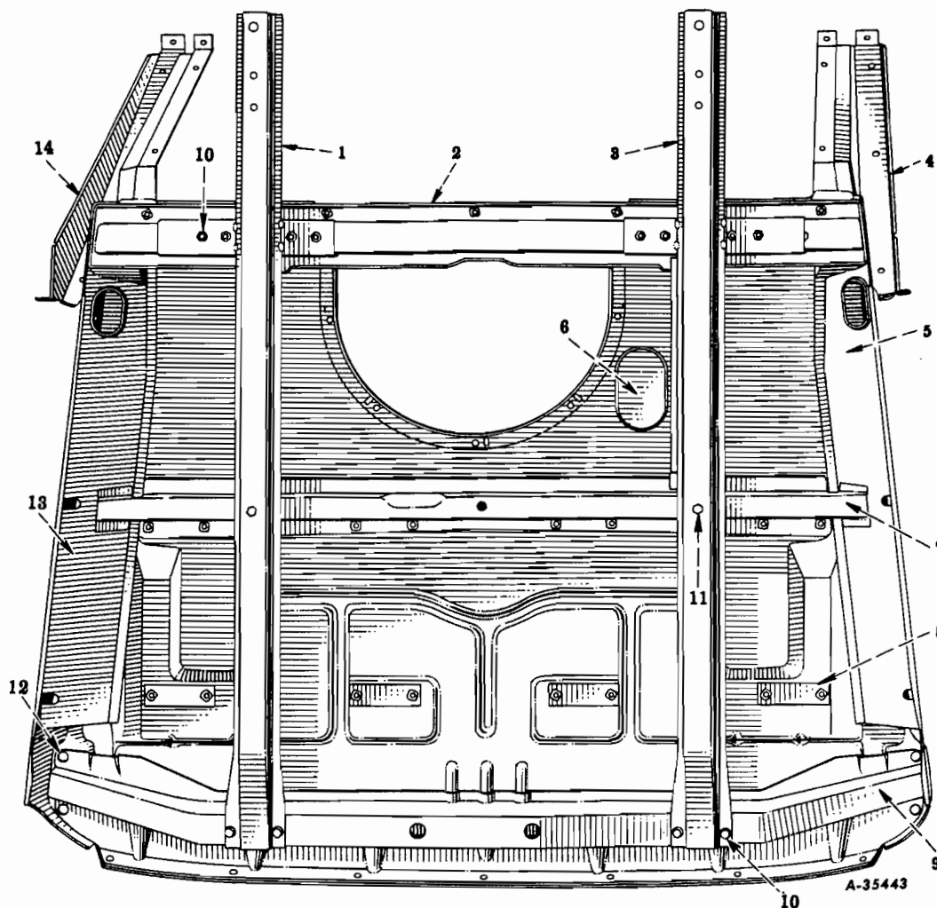
FIG. 16-16 – UNDERBODY ASSEMBLY (For Regular Cab Codes 1603, 1606, Panel Body Codes 1610, 1618, Travelall Body Codes 1616, 1617, 1619) (R-100, R-110, R-120, R-130, R-140-4x4, R-150, R-160, R-160-4x4 Series)
