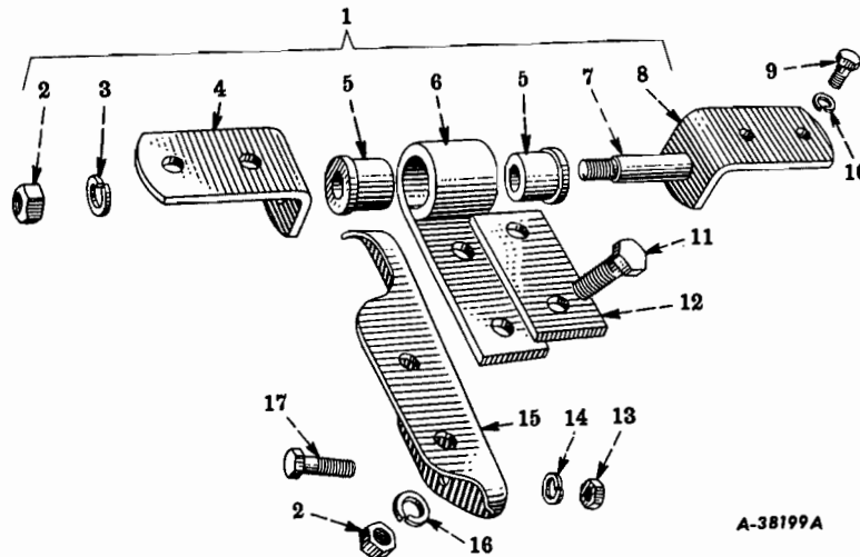
FIG. 16-2 - FRONT MOUNTING
