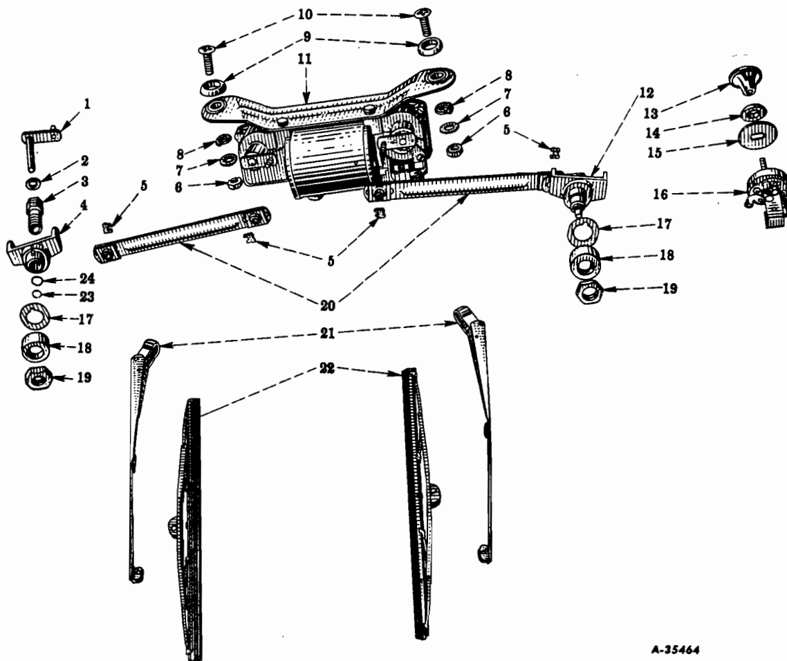
FIG. 16-47 - DUAL ELECTRIC WINDSHIELD WIPERS (Code 1692)
