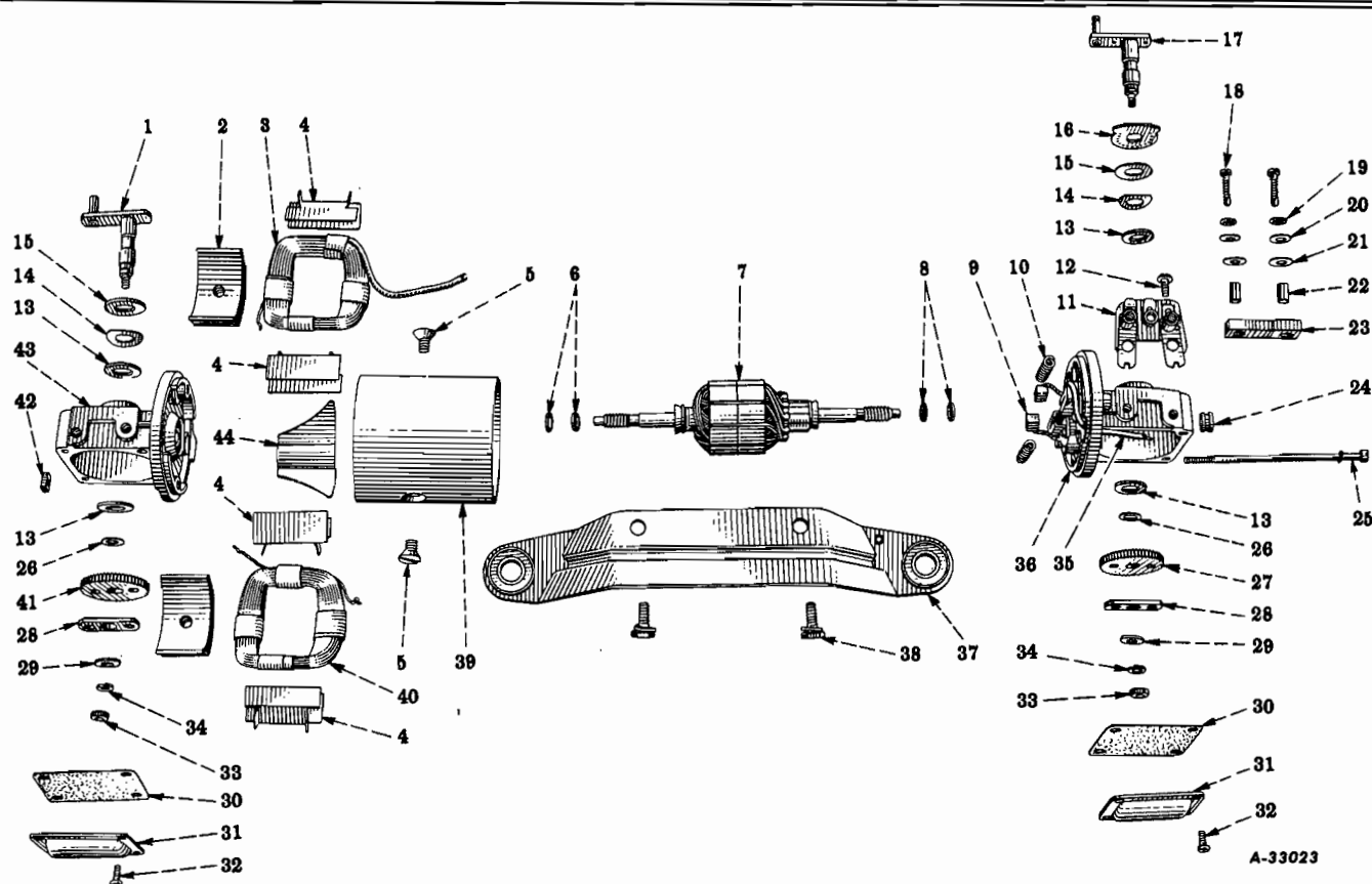
FIG. 16-48 — ELECTRIC WINDSHIELD WIPER MOTOR (American Bosch) (Cade 1692)
