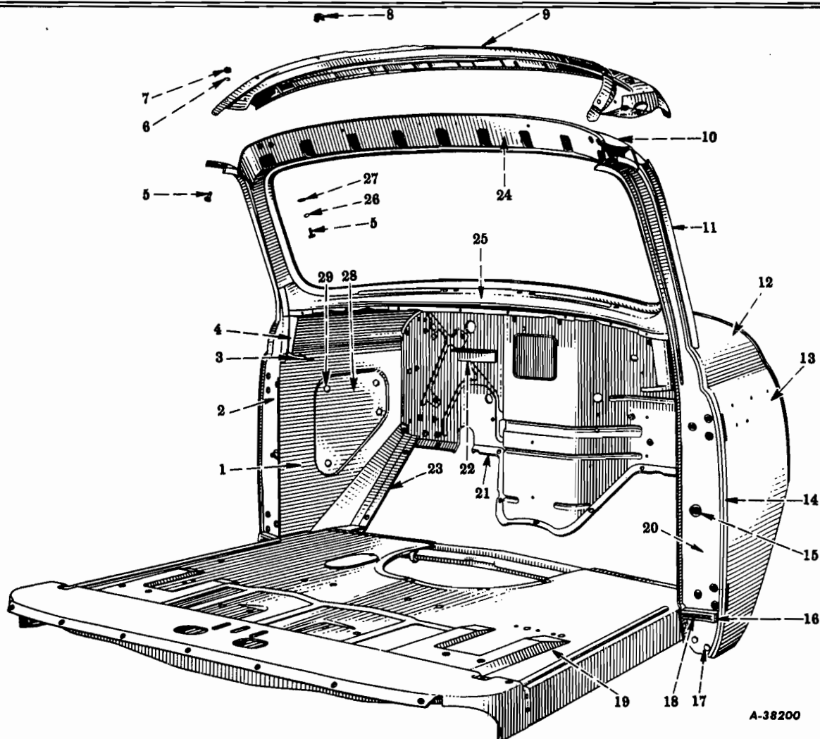
FIG. 16-14 - CAB COWL AND UNDERBODY (Codes 1603, 1606, 1610, 1616, 1617, 1618, 1619) (R-100, R-110, R-120, R-130, R-140-4x4, R-150, R-160, R-160-4x4 Series)
