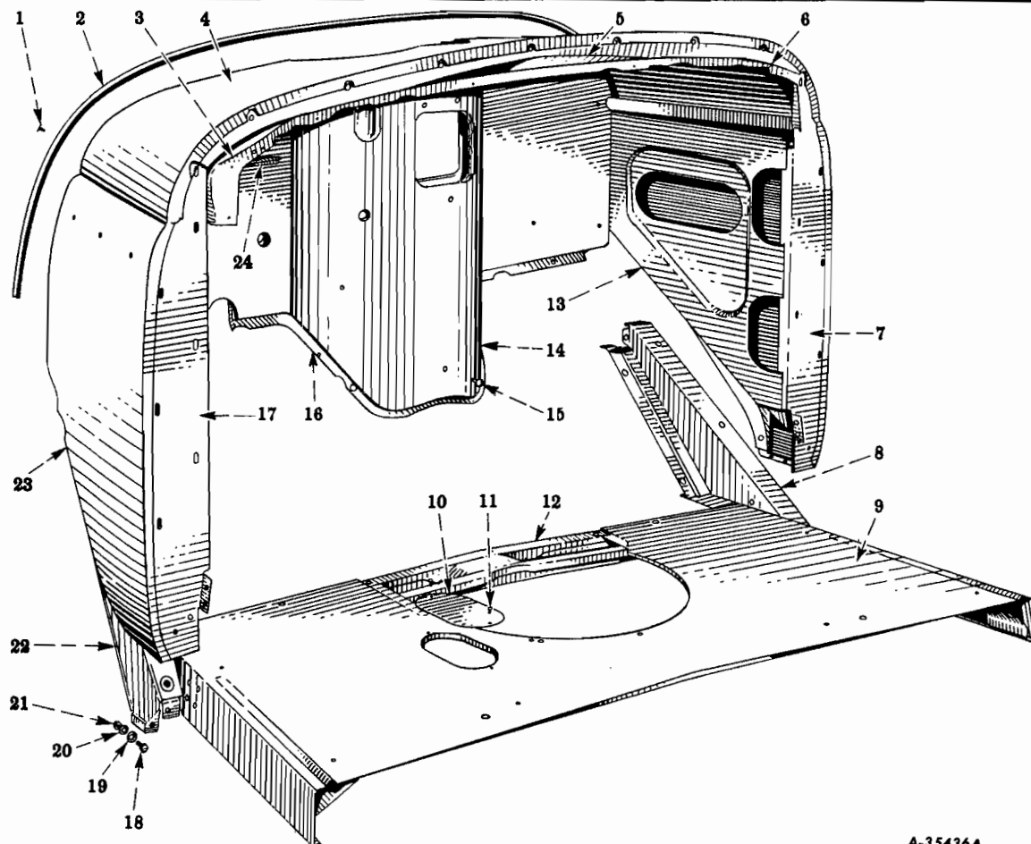
FIG. 16-8 - FLAT BACK COWL (Code 1601)
