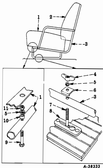
FIG. 16-39 — PASSENGER SEAT (Center and Rear) (For Travelall Body Codes 1616, 1617, 1619)
