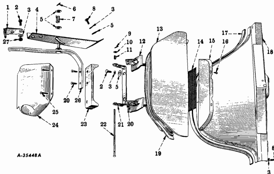
FIG. 16-19 - COWL VENTILATOR
