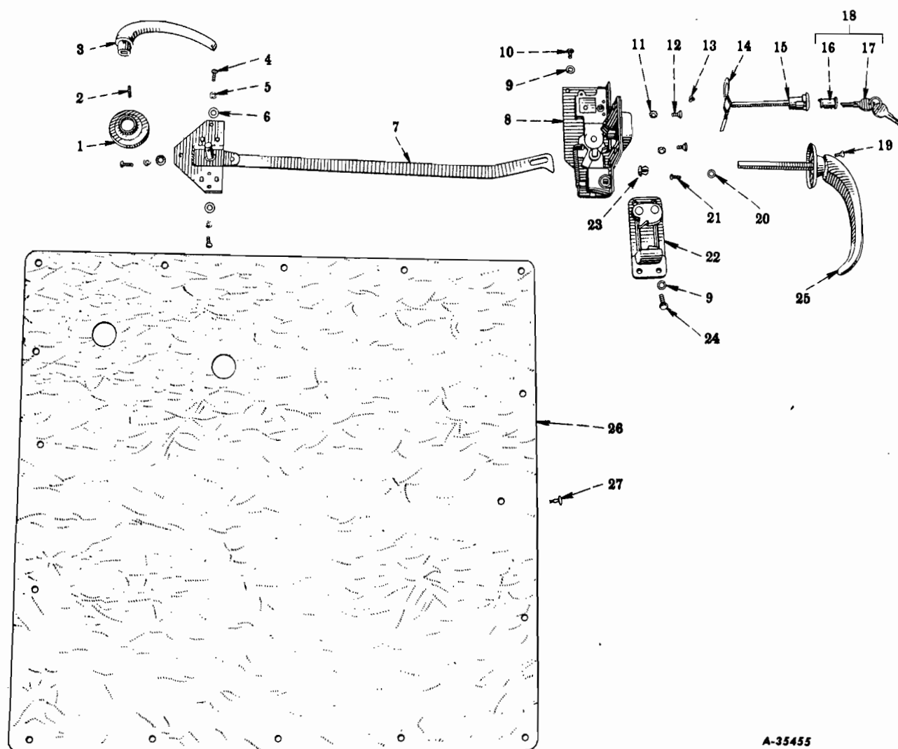
FIG. 16-29 – CAB DOOR TRIM, LOCK AND LATCH (For Codes 1603, 1610, 1613, 1616, 1617) (Below R-100-19474, R-110-53455, R-120-11688, R-130-10102, R-140-4x4-1053, R-150-3844, R-160-32760, R-160-4x4-947, RC-160-2997)
