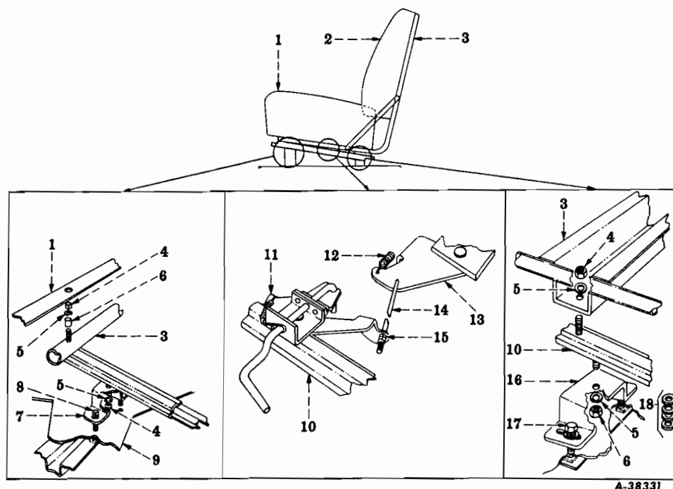
FIG. 16-37 — DRIVER'S SEAT (For Travelall Body Codes 1616, 1617, 1619)
