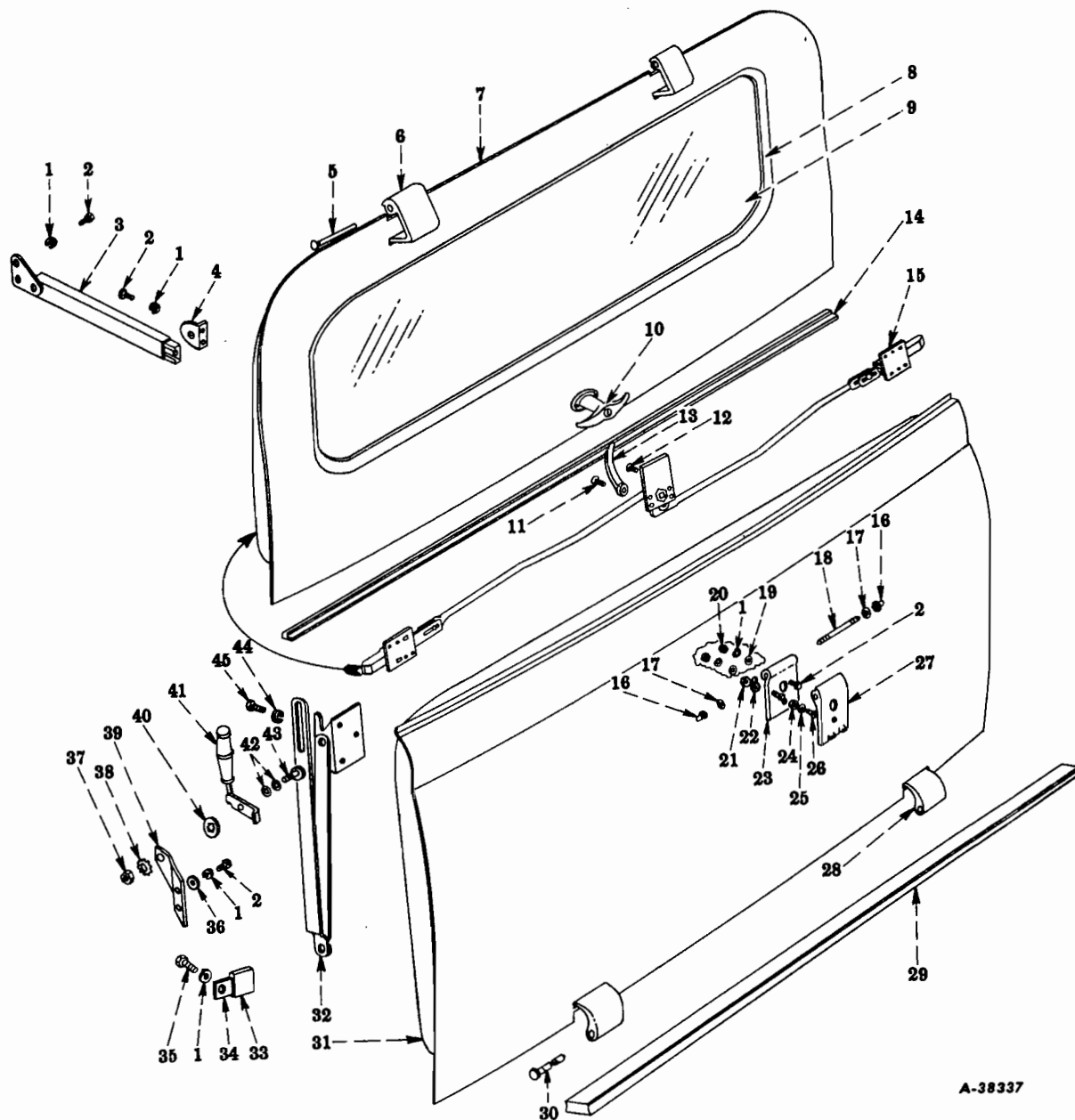
FIG. 16-44 – TAILGATE AND LIFTGATE (For Travelall Body Codes 1616, 1619)
