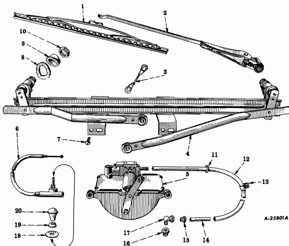
FIG. 16-46 — VACUUM WINDSHIELD WIPER
