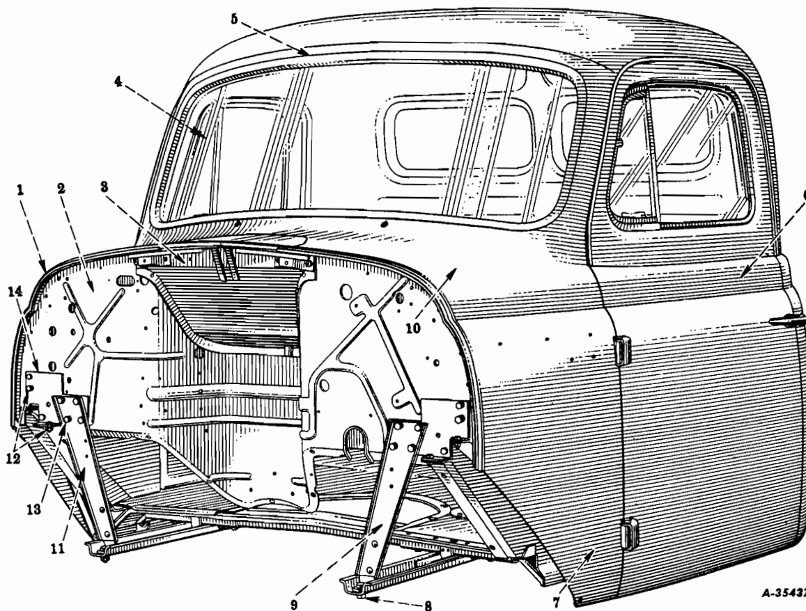
FIG. 16-10 - CAB ASSEMBLY (Code 1603, 1606) (Left Front View) (R-100, R-110, R-120, R-130, R-140-4x4, R-150, R-160, R-160-4x4 Series)
