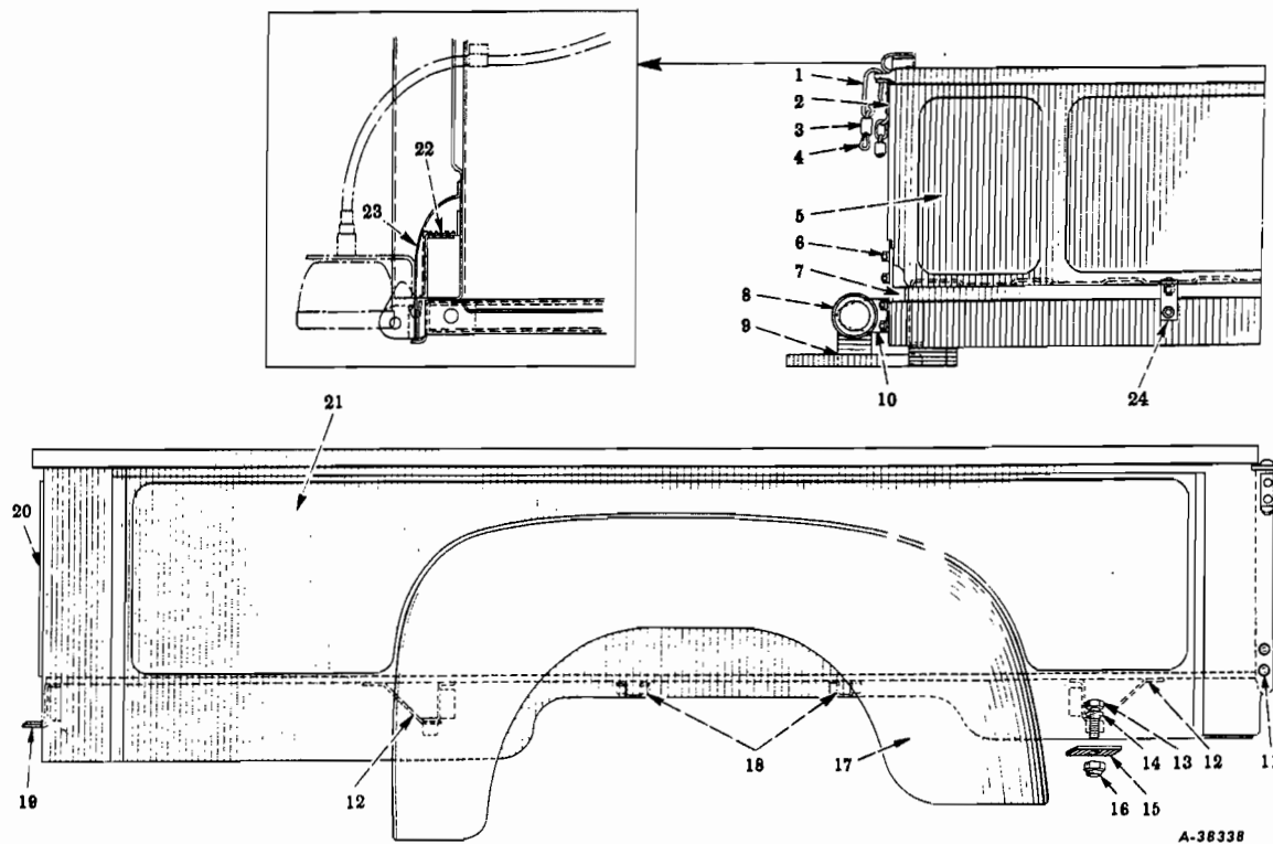
FIG. 16-45 — PICKUP BODY
