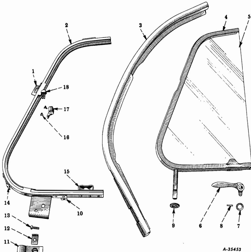
FIG. 16-27 - DOOR VENT WINDOW (Excel Corp.) (For Codes 1603, 1610, 1613, 1616, 1617) (Below R-100-19474, R-110-53455, R-120-11688, R-130-10102, R-140-4x4-1053, R-150-3844, R-160-32760, R-160-4x4-974, RC-160-2997) (Optional With Fig. 16-28)
