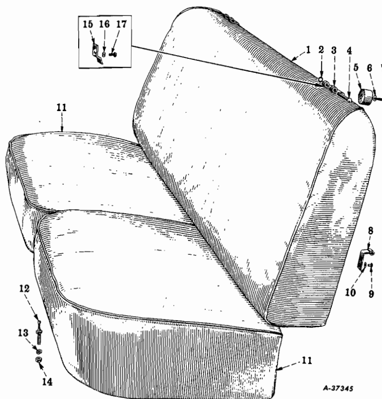
FIG. 16-35 — FULL WIDTH BACK CUSHION AND DIVIDED SEAT (Spring Type Standard - Rubber Type Code 1674) (RC-160)
