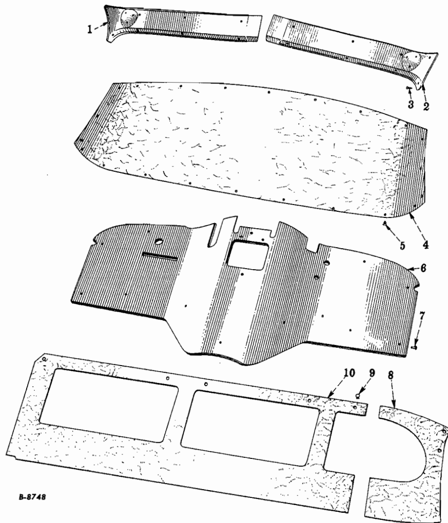
FIG. 16-32 — HEADER PANELS, ROOF TRIM, SIDE TRIM AND DASH INSULATOR (For Travelall Body Codes 1616, 1617, 1619)
