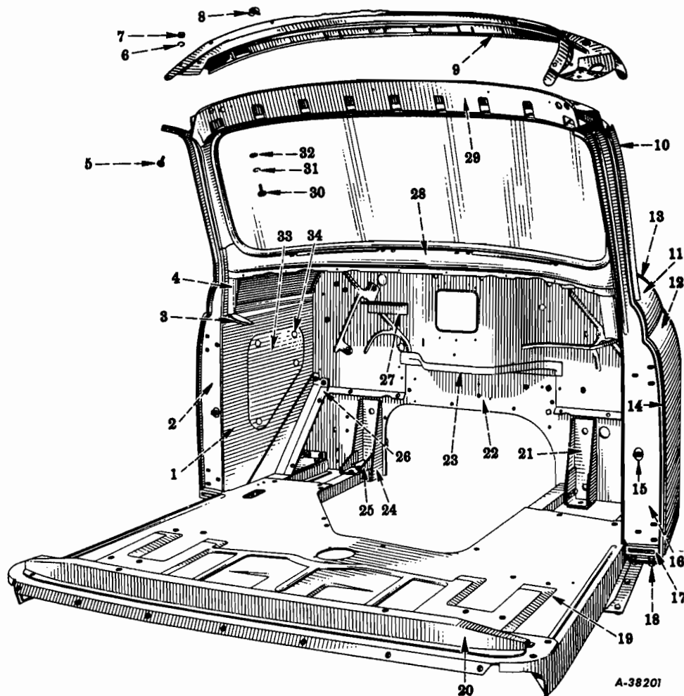
FIG. 16-15 - CAB COWL AND UNDERBODY (Code 1606, 1613) (RC-160)
