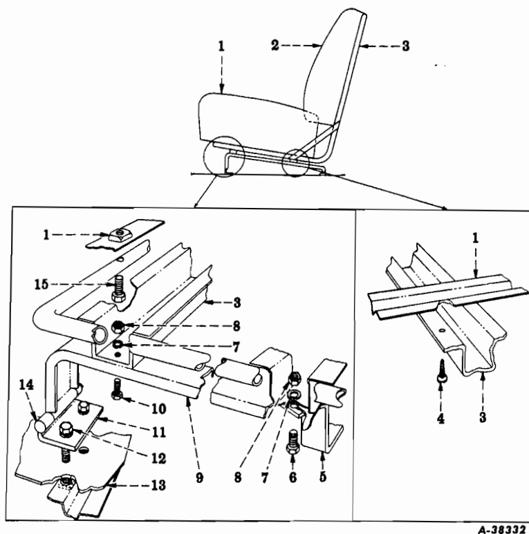
FIG. 16-38 — PASSENGER SEAT (Front) (For Travelall Body Codes 1616, 1617, 1619)
