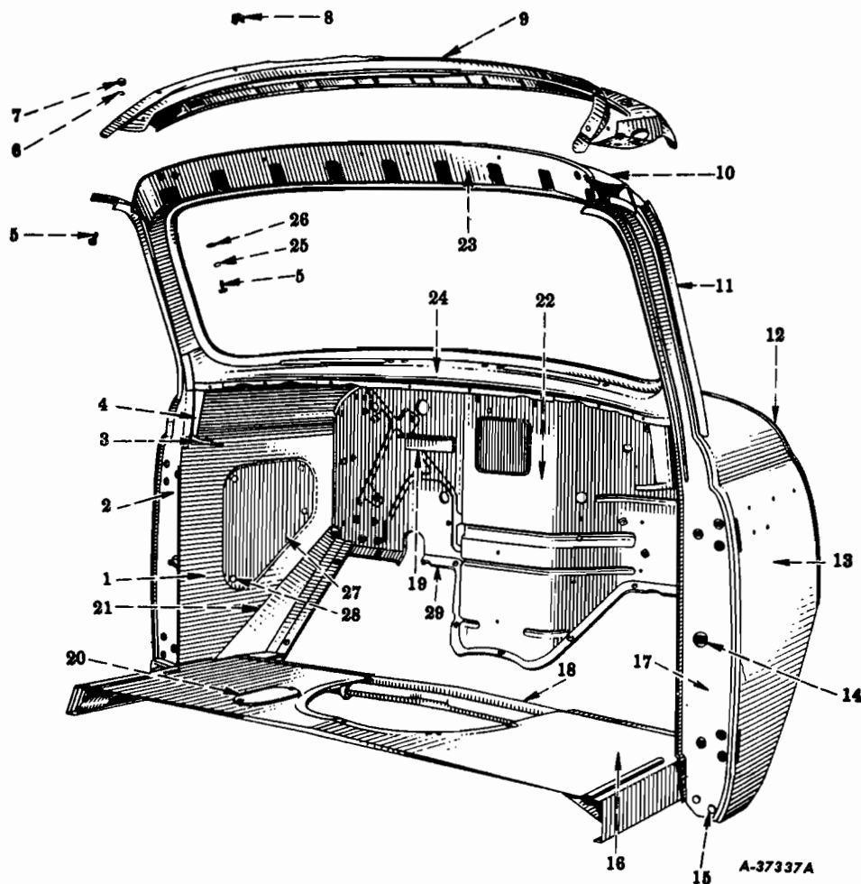
FIG. 16-9 – FRONT END SECTION (Code 1602) (R-110, R-120, R-130, R-140-4x4, R-150, R-160, R-160-4x4 Series)
