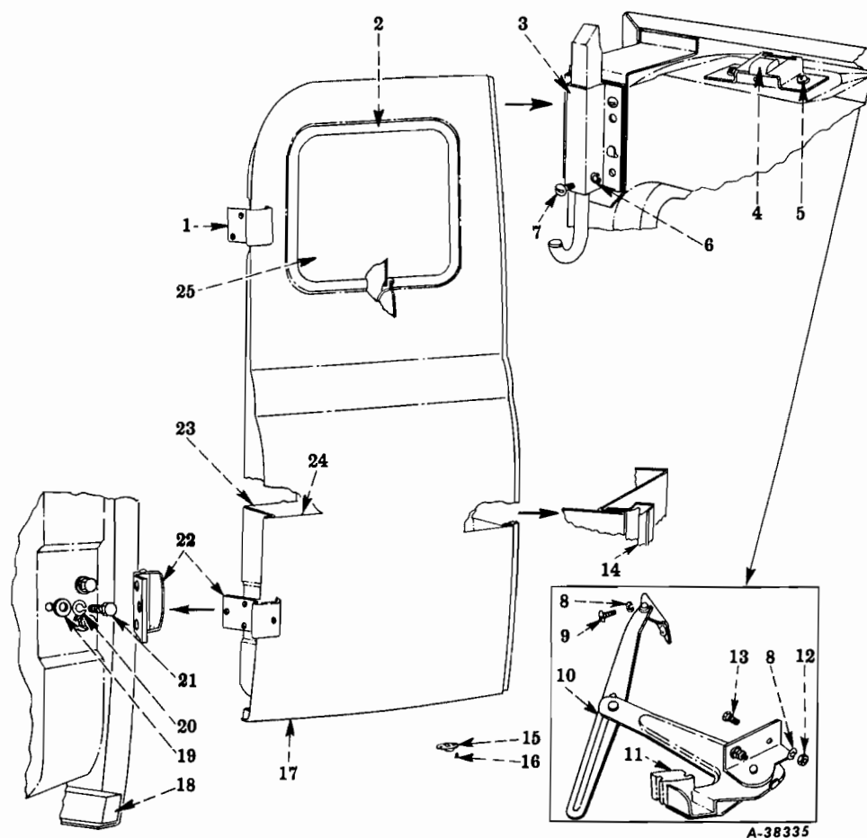
FIG. 16-41 — LEFT REAR DOOR (For Panel Body Codes 1610, 1618 and Travelall Body Code 1617)
