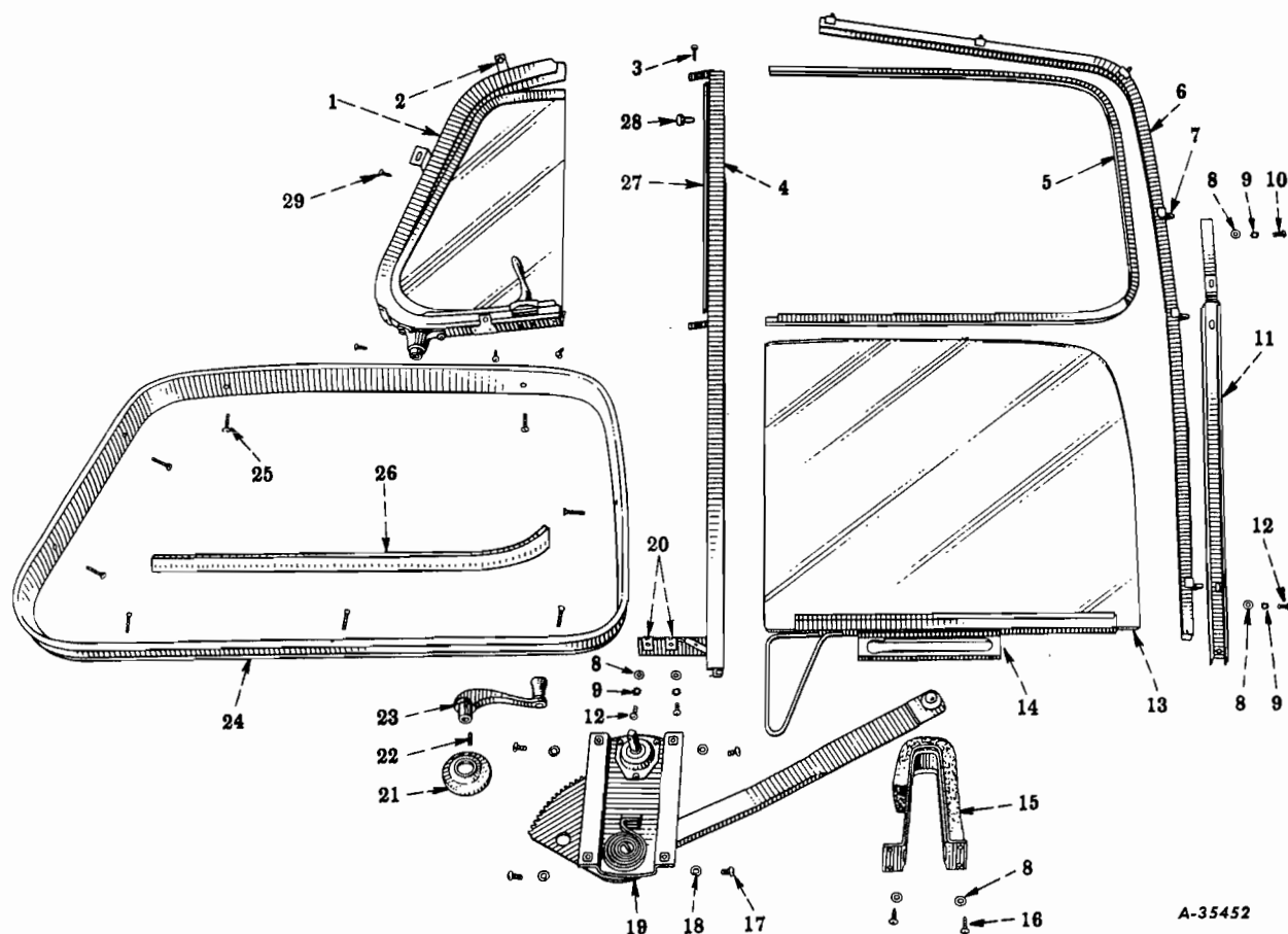
FIG. 16-25 - CAB DOOR WINDOW (For Codes 1603, 1610, 1613, 1616, 1617) (Below R-100-19474, R-110-53455, R-120-11688, R-130-10102, R-140-4x4-1053, R-150-3844, R-160-32760, R-160-4x4-974, RC-160-2997)
