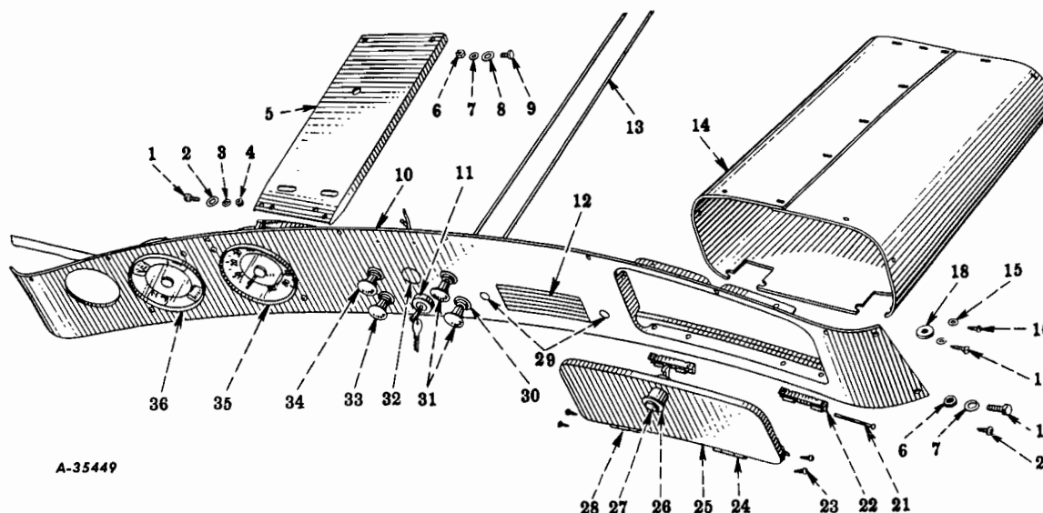
FIG. 16-20 - INSTRUMENT PANEL AND GLOVE BOX
