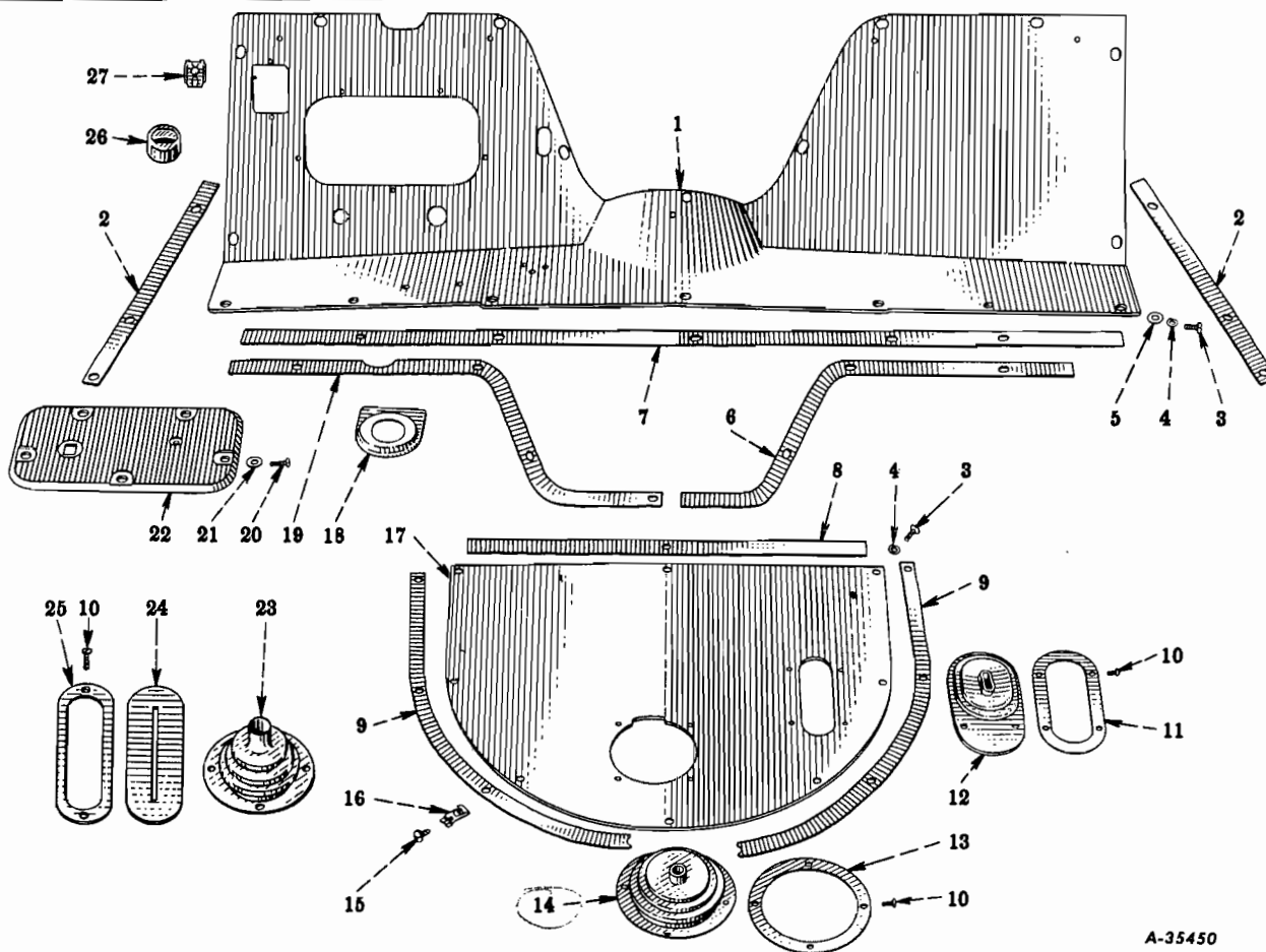
FIG. 16-21 – CAB TOE-BOARD AND COVER PLATE (R-100, R-110, R-120, R-130, R-140-4x4, R-150, R-160, R-160-4x4 Series)
