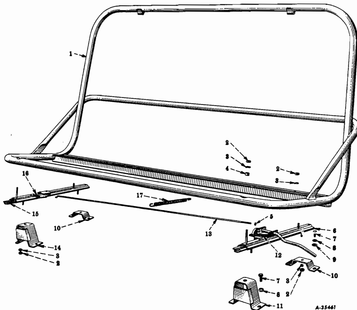
FIG. 16-33 – FULL WIDTH SEAT FRAME AND MOUNTING PARTS (For Cab Codes 1603, 1606, 1613)
