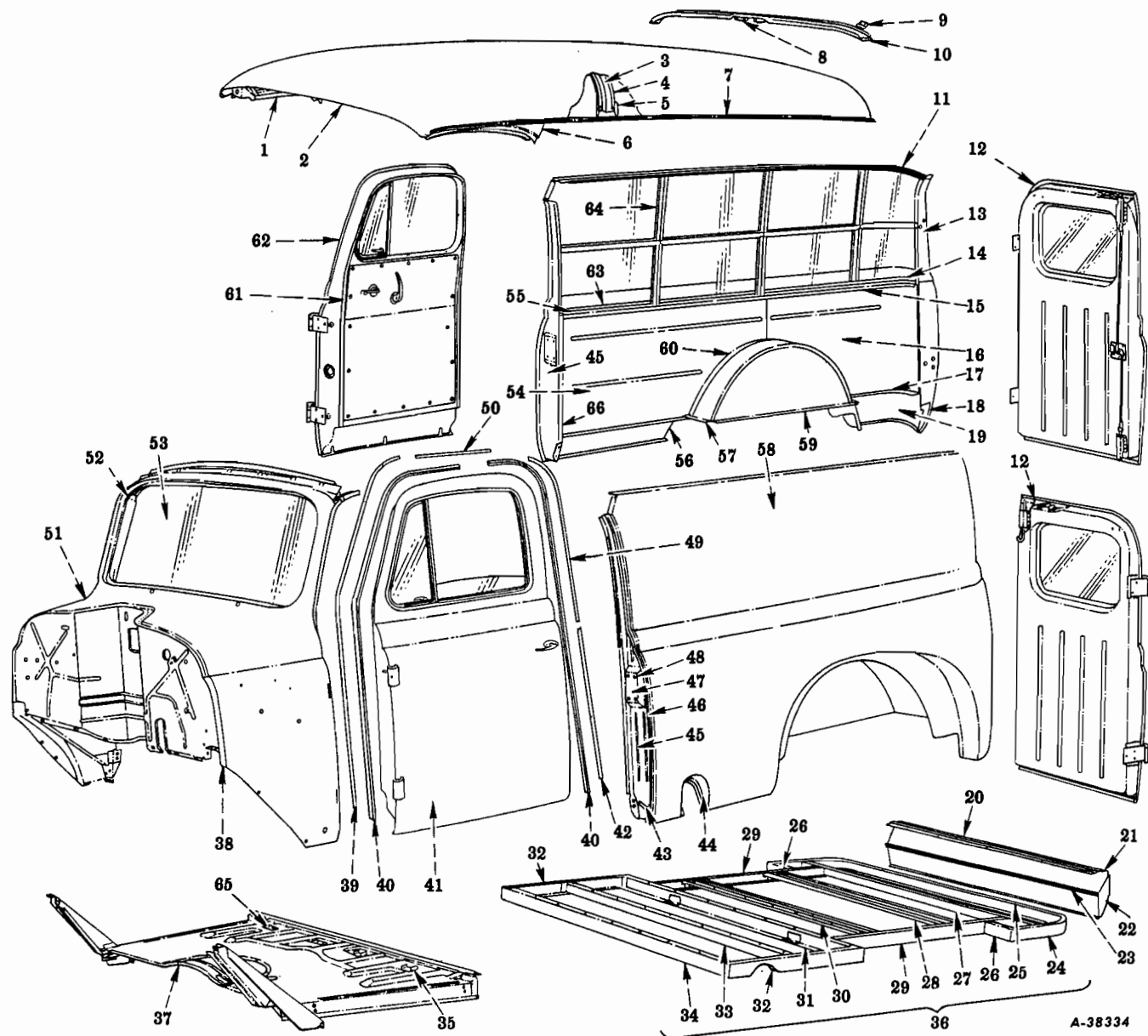
FIG. 16-40 — PANEL BODY ASSEMBLY (Codes 1610, 1618)
