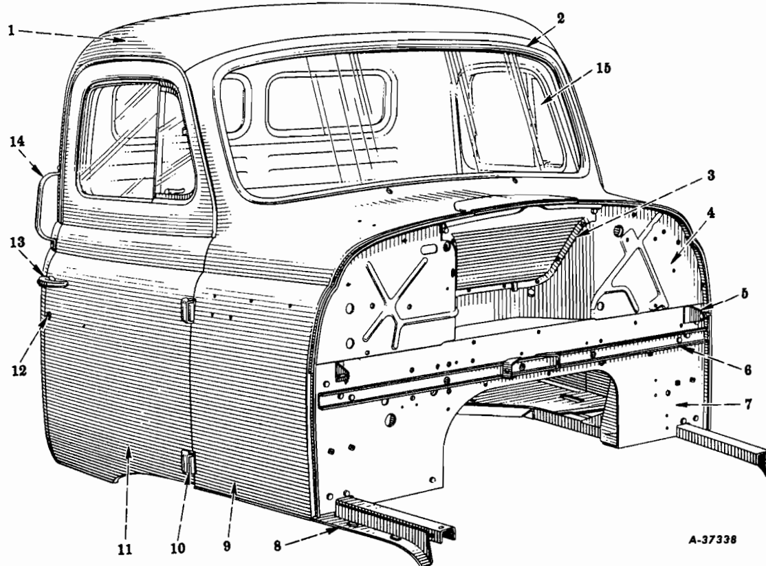
FIG. 16-11 – CAB ASSEMBLY (Codes 1606, 1613) (Right Front View) (RC-160)
