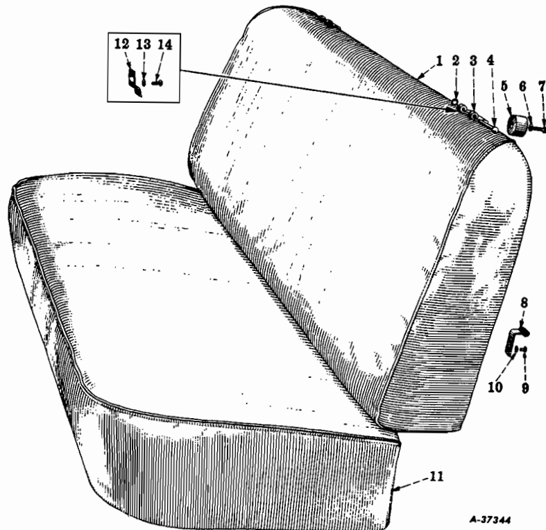
FIG. 16-34 — FULL WIDTH SEAT AND BACK CUSHIONS (For Cab Codes 1603, 1606) (Spring Type - Standard, Rubber Type - Codes 1673, 1674) (R-100, R-110, R-120, R-130, R-140-4x4, R-150, R-160, R-160-4x4 Series)
