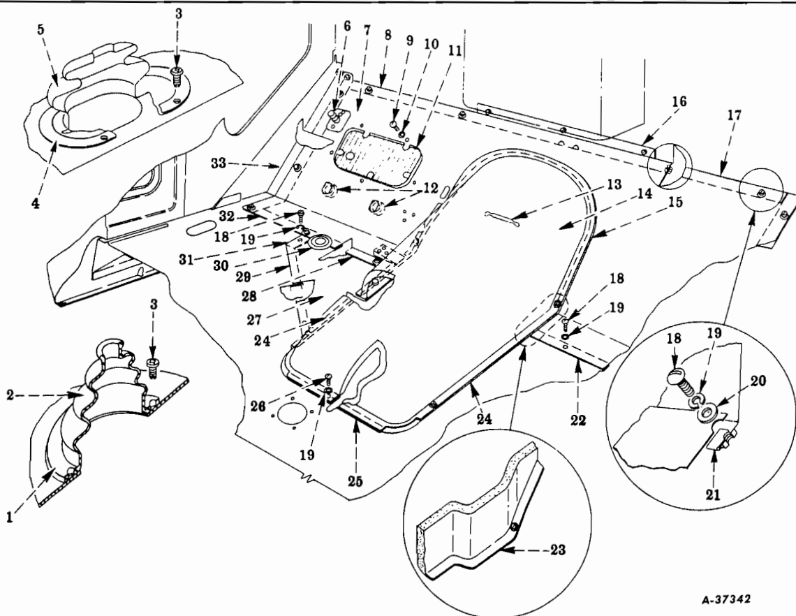
FIG. 16-22 - CAB TOE-BOARD AND COVER PLATE (RC-160)
