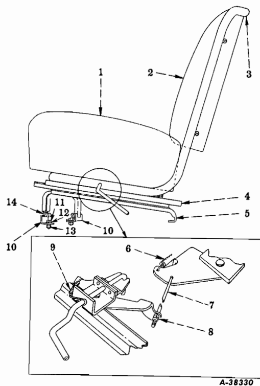
FIG. 16-36 — DRIVERS SEAT (For Panel Body, Codes 1610, 1618)
