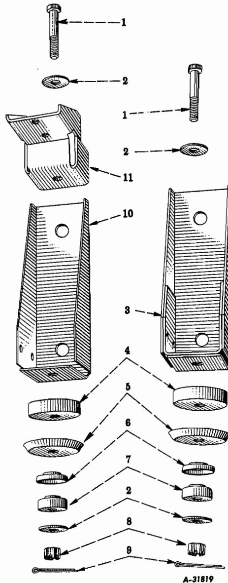
FIG. 16-3 – FRONT MOUNTING (For Cab Codes 1606, 1613) (RC-160)
