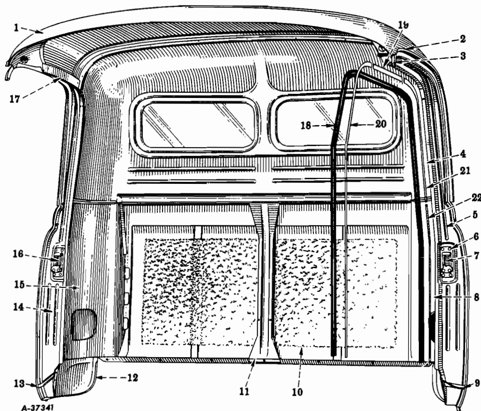
FIG. 16-18 - CAB ROOF AND BACK PANEL
